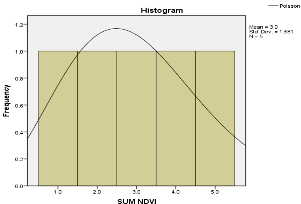
Figure 19. Sum NDVI of the Five Fields. Source: Author’s Labwork (2025)
