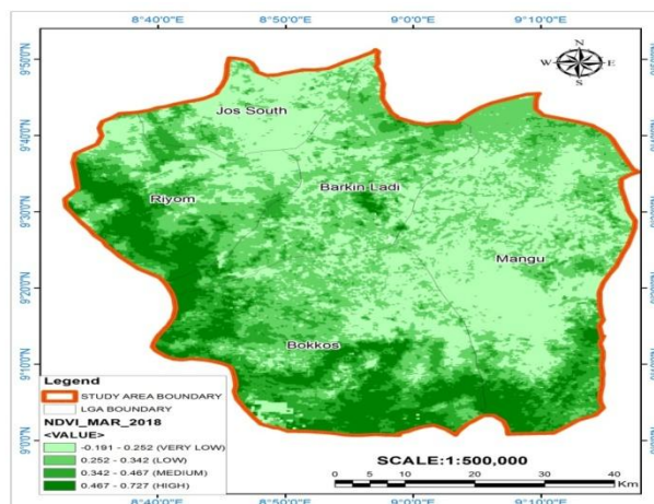
Figure 14. NDVI Value for March, 2018 of the Study Area.
